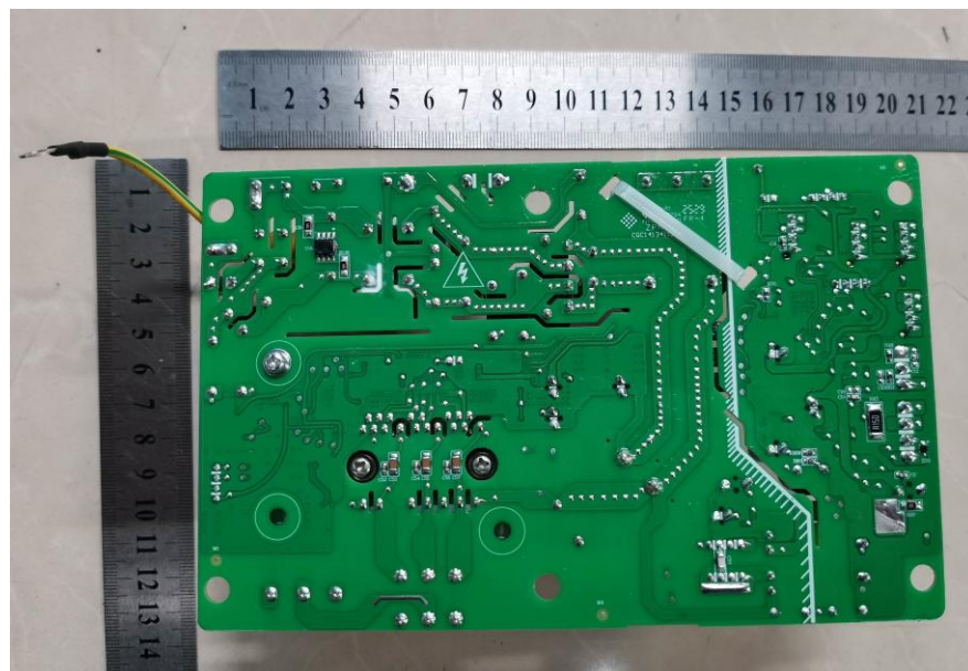
Internal construction
