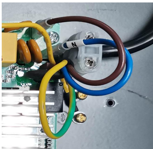
Internal construction
